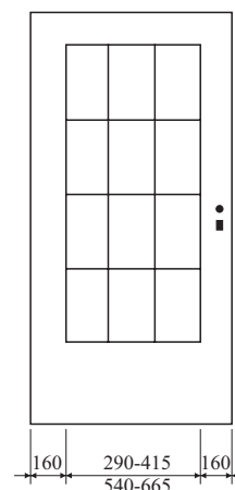
LA-M/EX (985)
