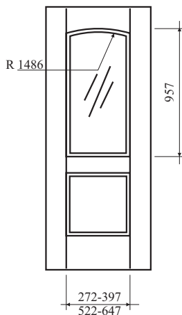
Modell SOAD.
