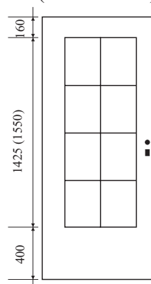
LA-M/EX (610-735-860)
